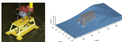
Validation of wave loading during an operation through the splash zone. Left: test set-up with instrumented model (MARIN shallow water basin). Right: ComFLOW simulation.
